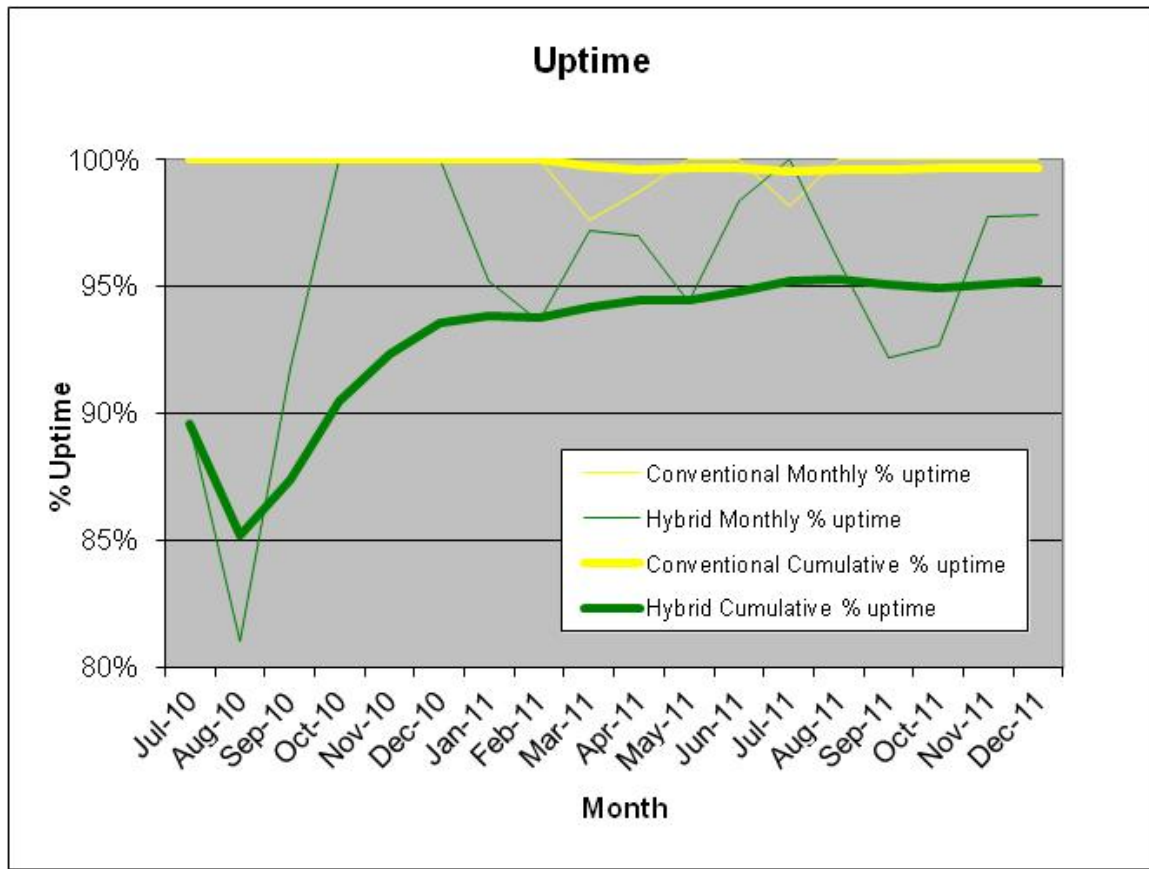
Figure 15. Cumulative uptime
