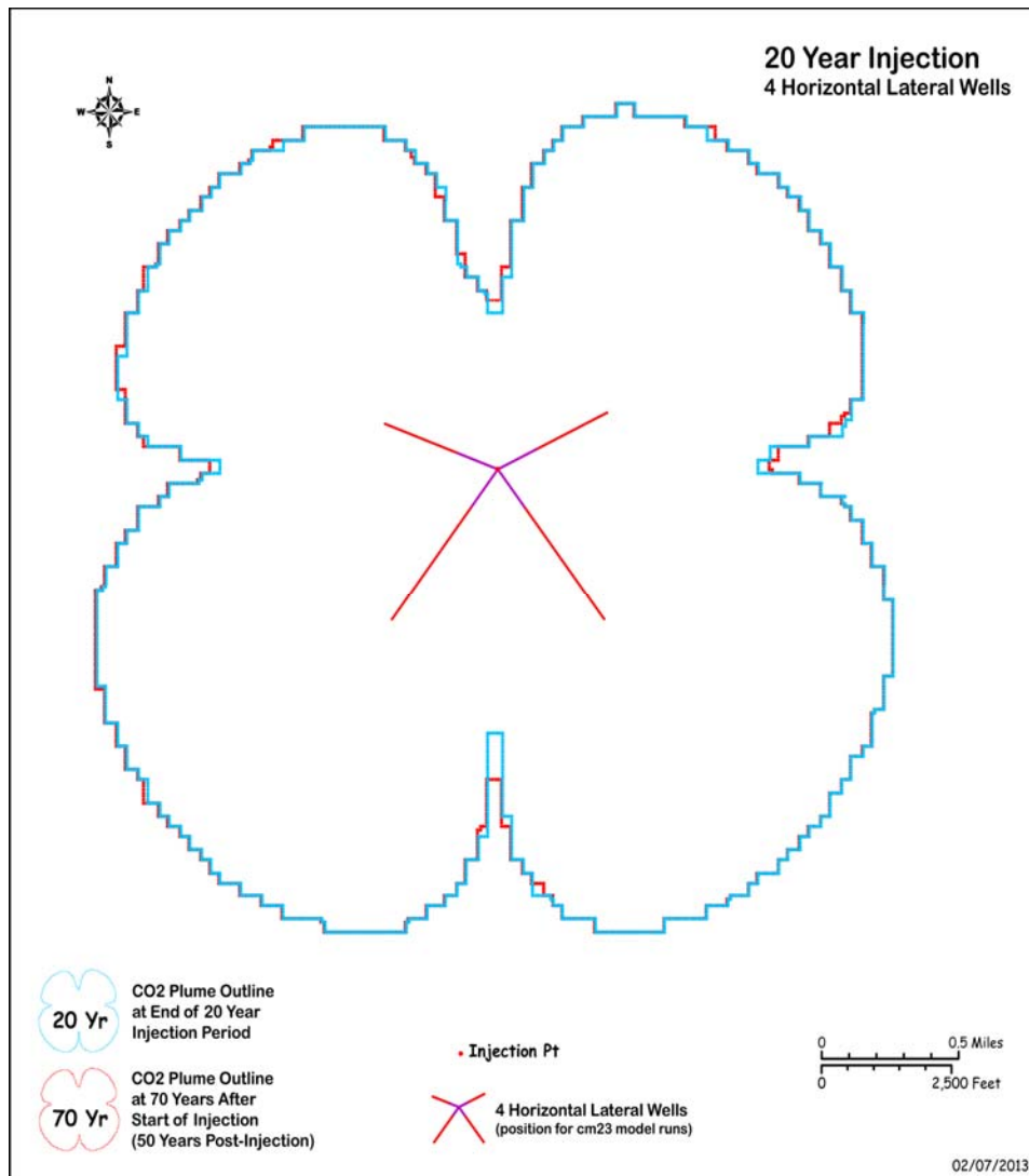
Figure S-14. Predicted Areal Extent of CO 2 Plume
