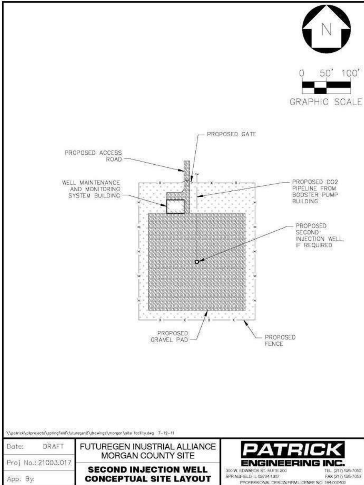
Figure S-11. Secondary Injection Well Site Surface Features Conceptual Layout
