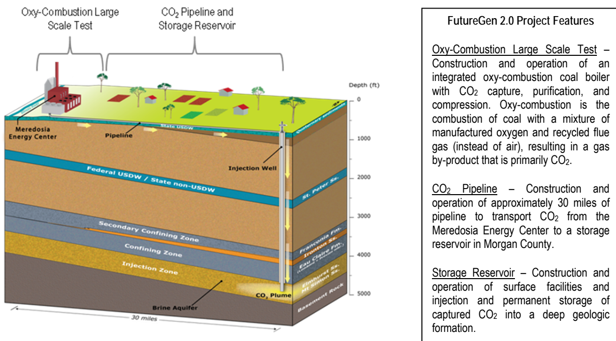
Figure S-1. The FutureGen 2.0 Project
