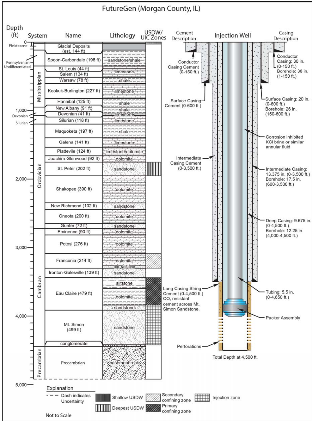
Figure S-12. Geological Stratigraphic Column for the CO 2 Storage Study Area and Proposed Vertical Injection Well Construction Details
