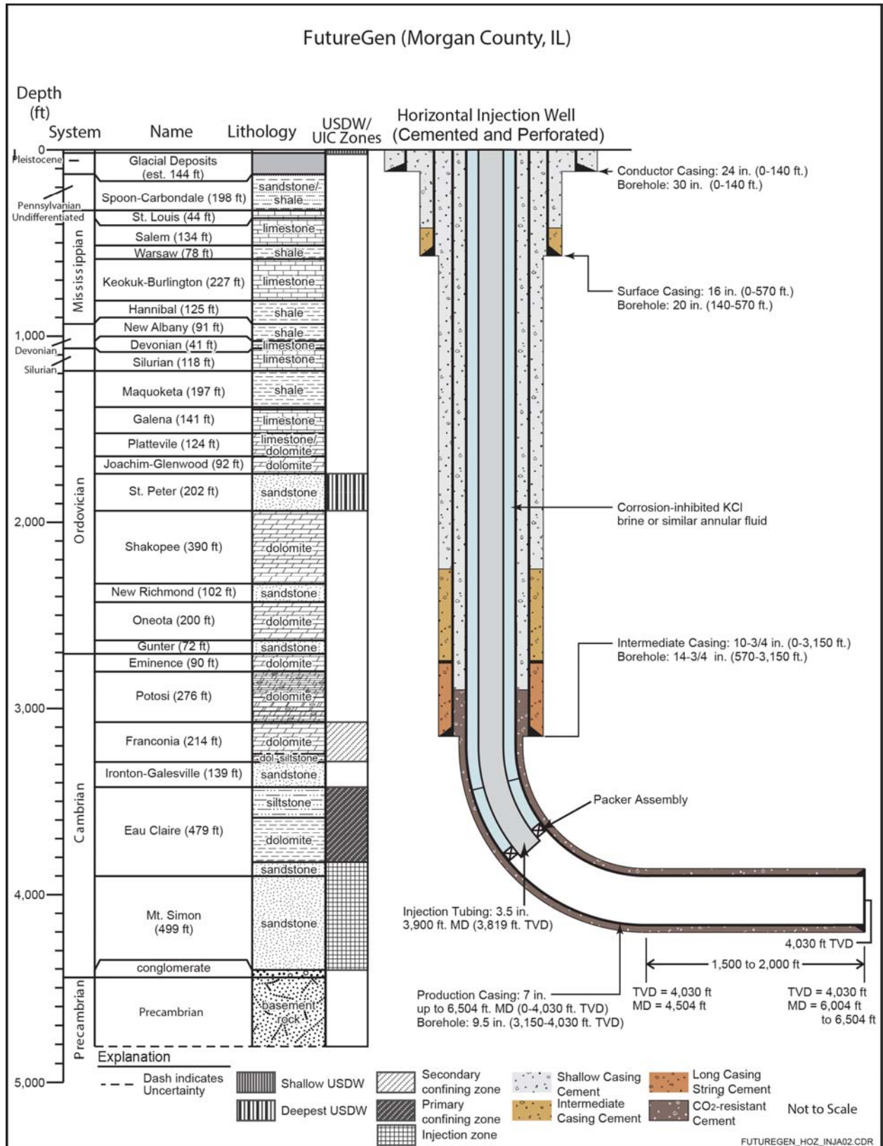
Figure S-13. Proposed Horizontal Injection Well Construction Details
