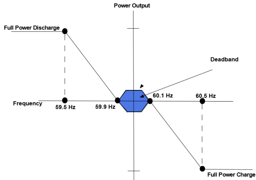
Figure 1. Potential Operating Mode for Battery Charging/Discharging
