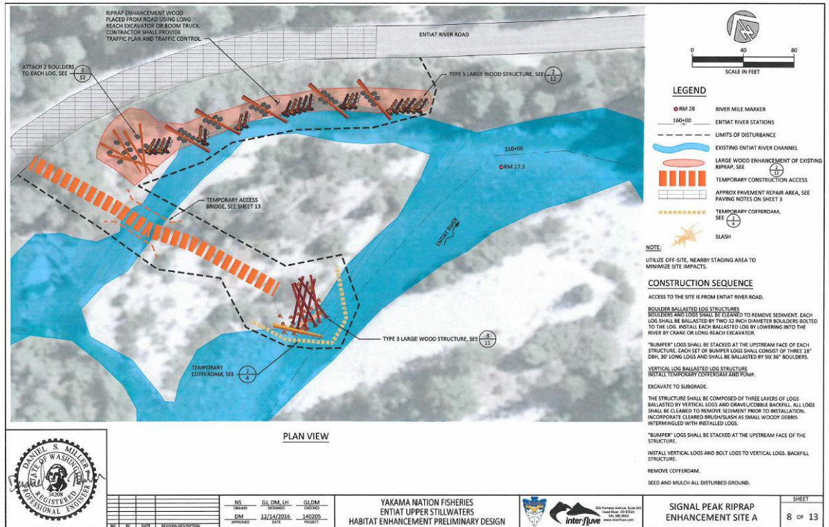
Figure 7. Signal Peak Riprap Enhancement Site A
