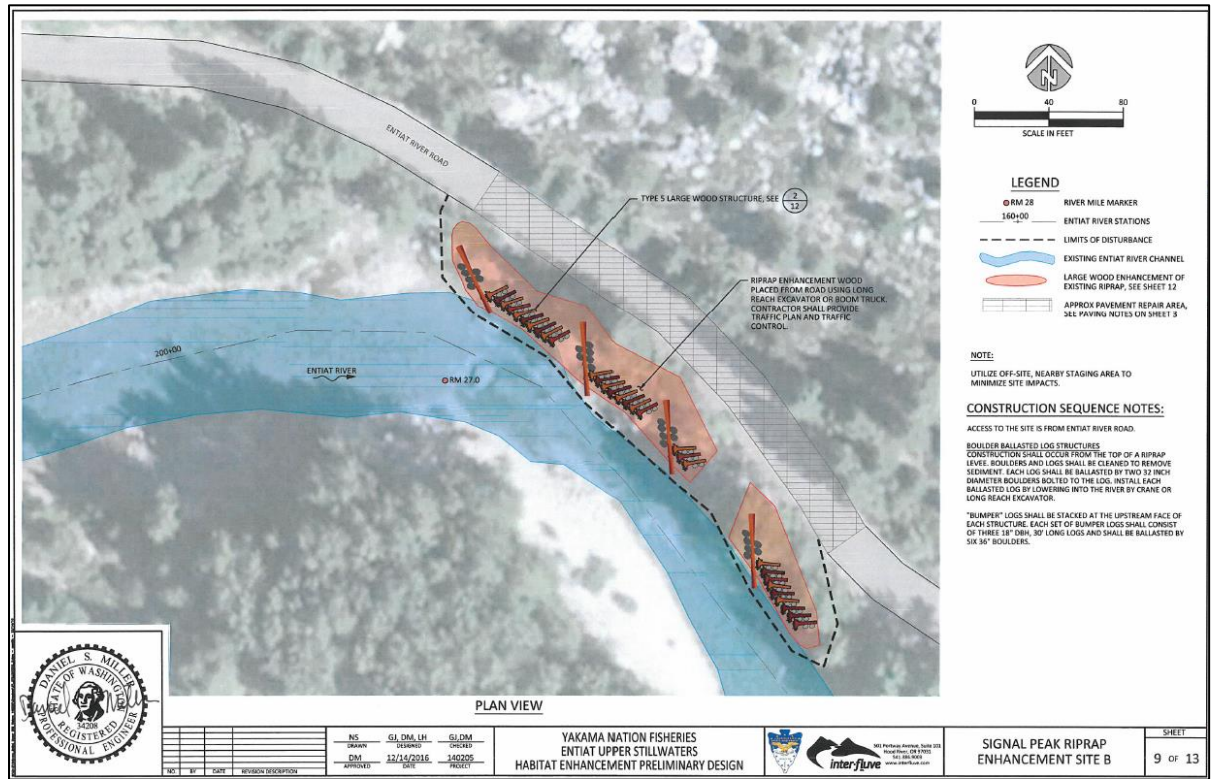
Figure 6. Signal Peak Riprap Enhancement Site B Design
