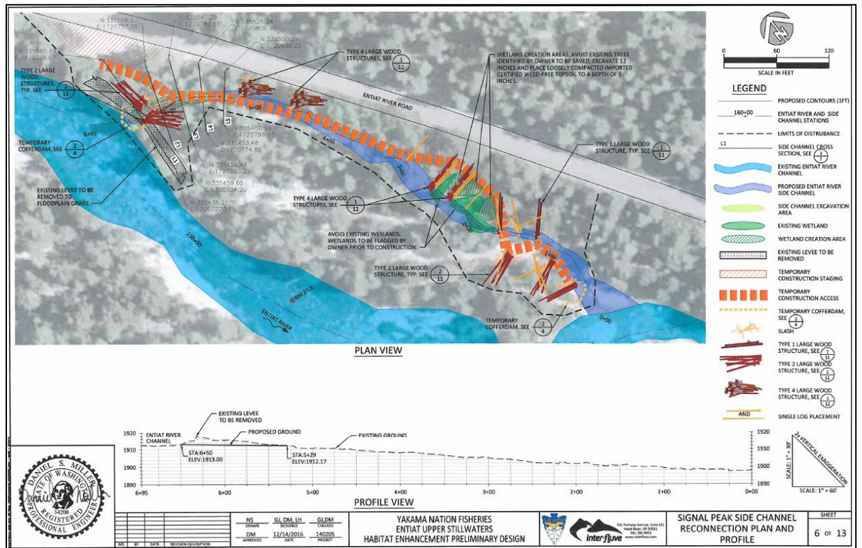
Figure 8. Signal Peak Side Channel Reconnection Design
