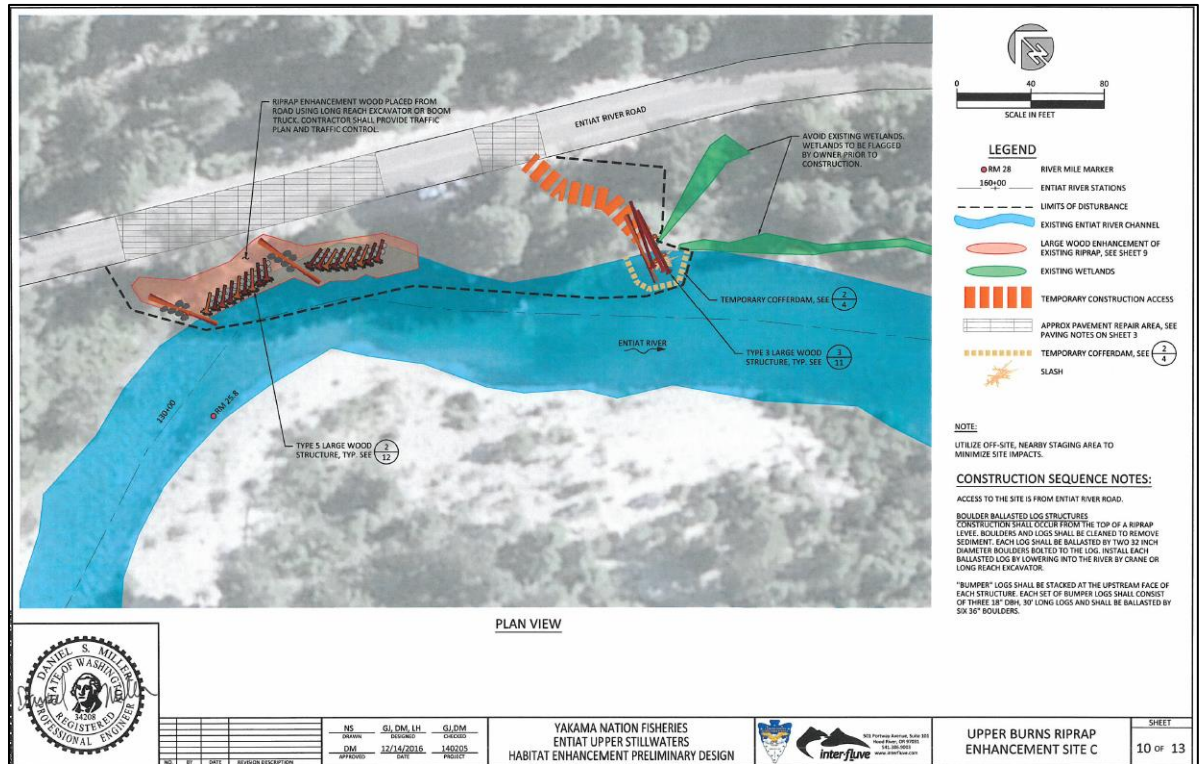
Figure 5. Upper Burns Riprap Enhancement Design
