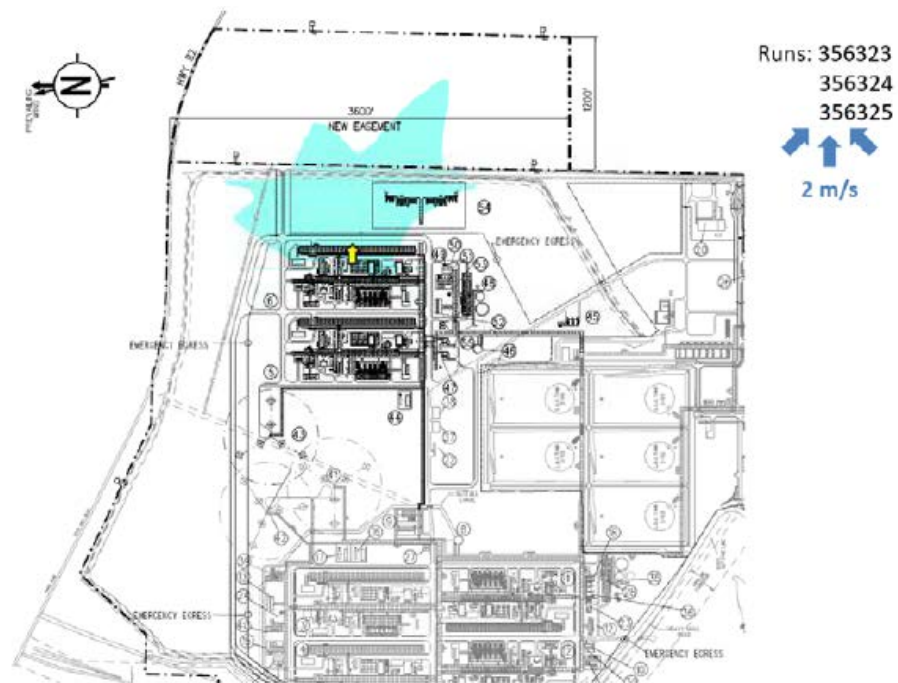
Figure 4 Propane Vapor Dispersion Zone – Flashing and Jetting
