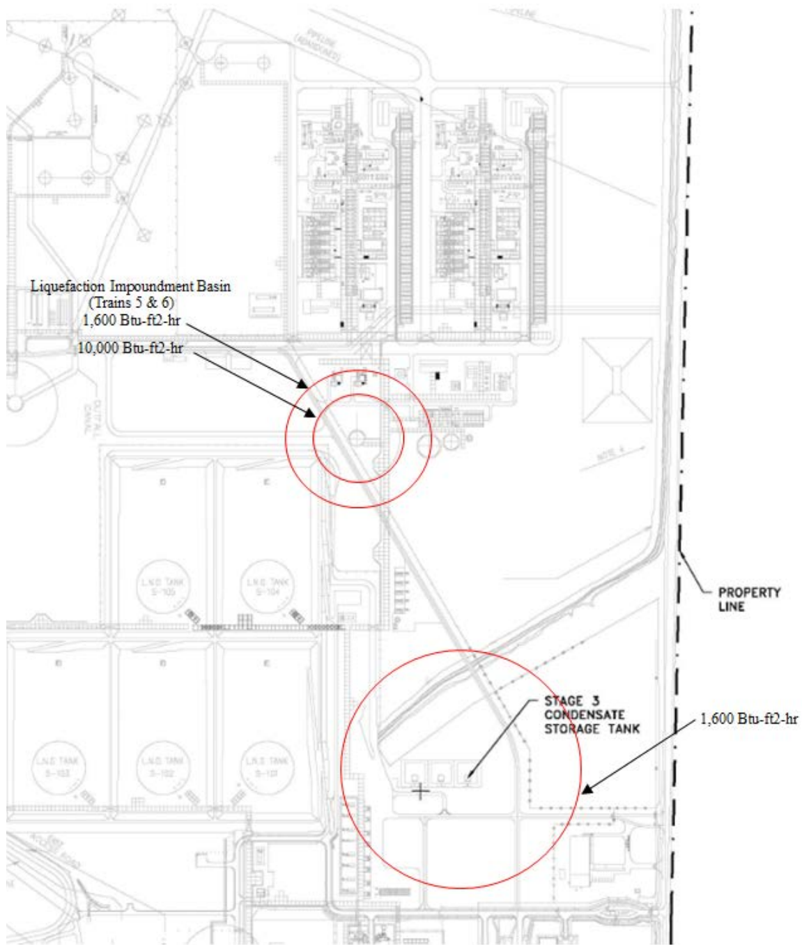
Figure 6 Thermal Radiation Distances (1,600 Btu-ft 2 -hr) for the LNG Impoundment Basin (Trains 5 & 6) and Condensate Storage Tank Area
