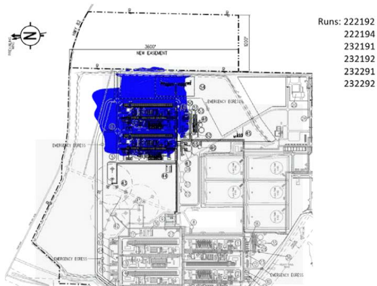
Figure 5 Extent of 1 Psi Overpressures due to Ethylene Design Spill in Train 6 – Shown as Shaded Areas
