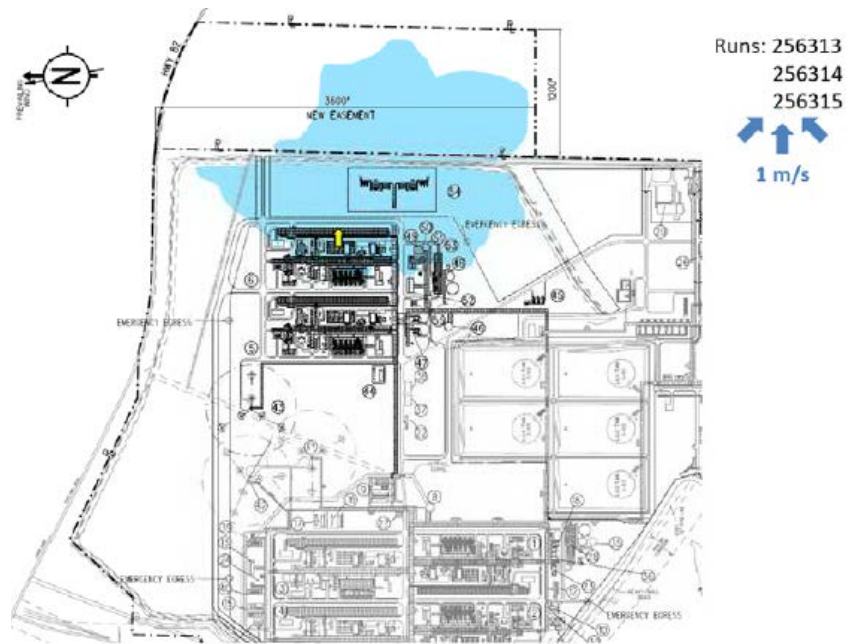
Figure 3 Ethylene Vapor Dispersion Zone – Flashing and Jetting
