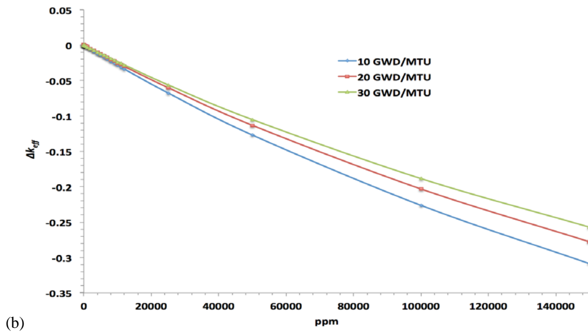
Figure 2-32. Reactivity impact of Cl concentration in groundwater: a) for different levels of neutron absorber; (b) for degraded basket configuration with different burnup levels.
