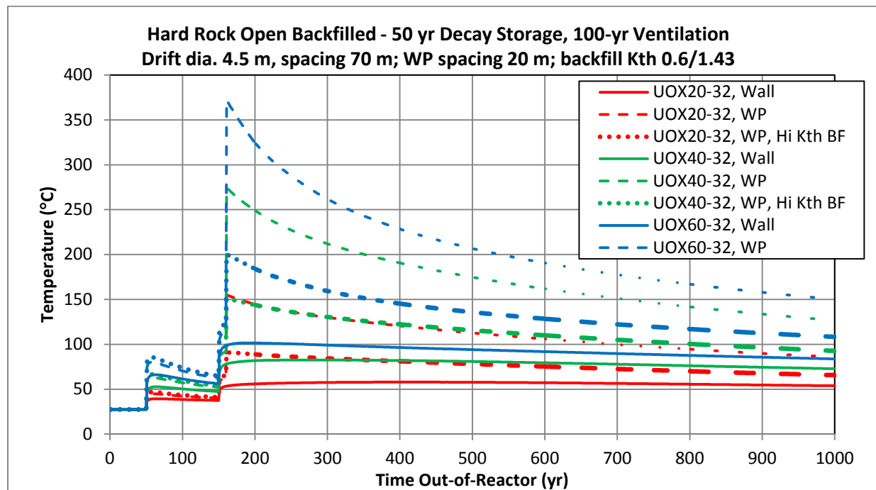
Figure 2-11. Thermal analysis of DPC disposal in a hard-rock backfilled, open-type repository with 50-yr decay storage, 100-yr ventilation, and both typical and high thermal conductivity backfill.
