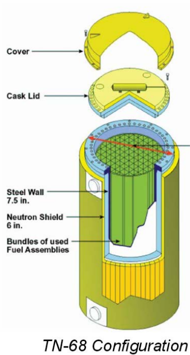
Figure 1-2. Example of bare fuel in a bolted cask (from Williams 2013).
