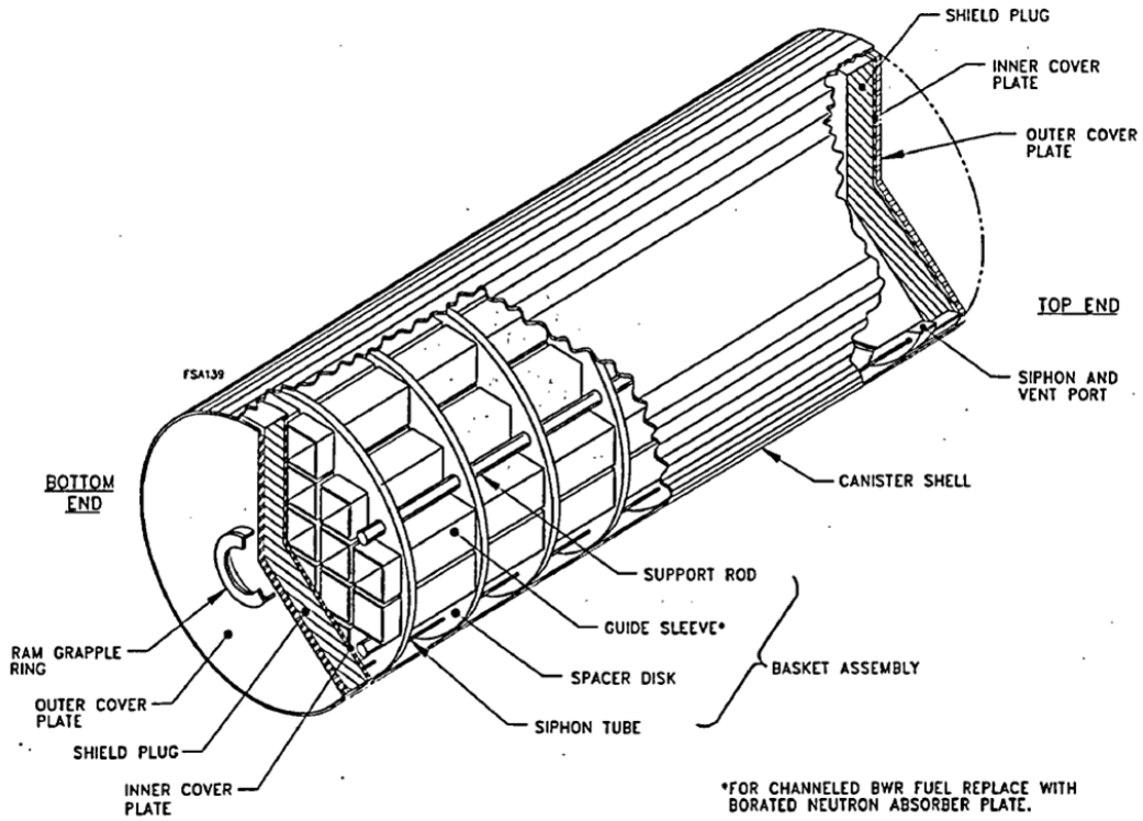
Figure 1-3. Representative design of DPC canister. NUHOMS 24PHB shown.
