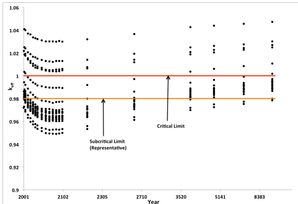
Figure 2-36. k_{eff} vs calendar year for the Site C basket degradation case based on actual loading.
