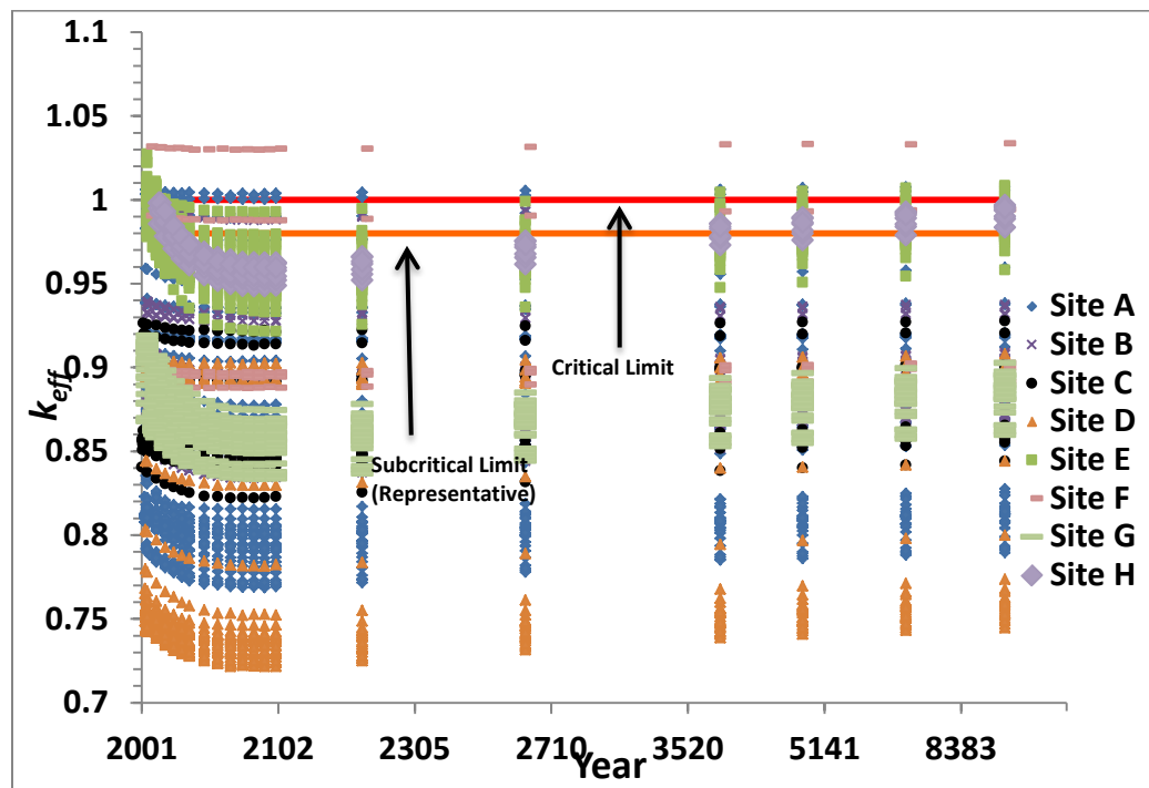
Figure 2-35. k_{eff} vs calendar year for the loss-of-neutron-absorber case based on actual loading.
