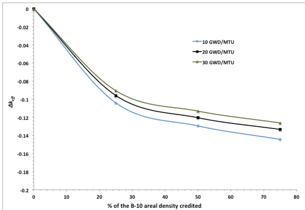
Figure 2-31. Reactivity impact of 10 B areal density variation.
