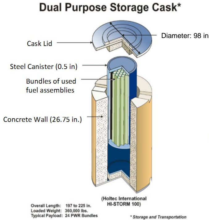
Figure 1-1. Example of a dual-purpose canister inside a storage overpack (cask) (modified from Easton 2011).
