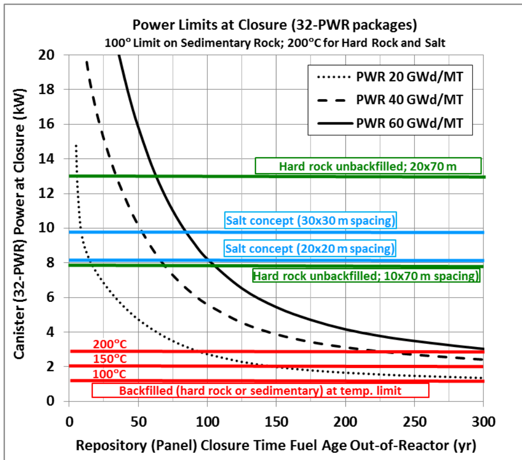
Figure 2-29. Heat output vs. age for a 32-PWR DPC, for three values of burnup (20, 40 and 60 GW-d/MT) showing approximate power limits (at repository closure) for different disposal concepts.
