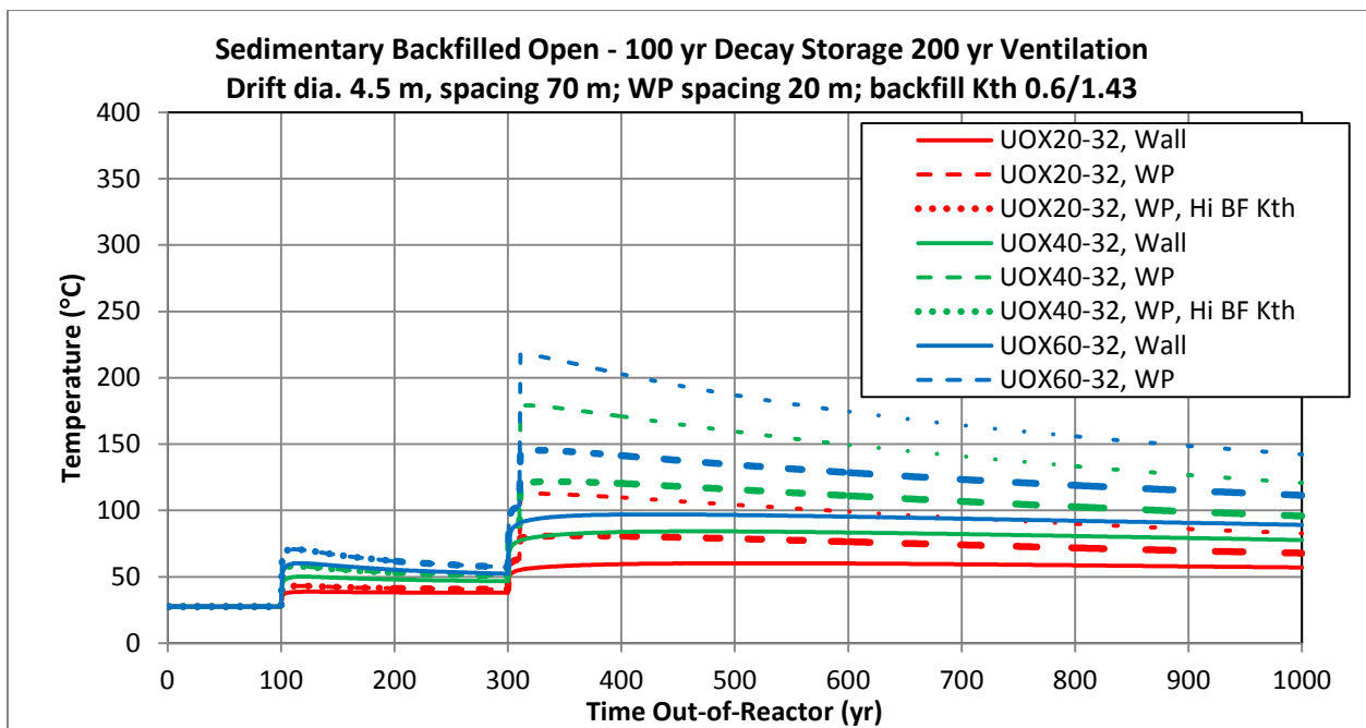
Figure 2-14. Thermal analysis of DPC disposal in a sedimentary backfilled, open-type repository with 100-yr decay storage and 200-yr ventilation.
