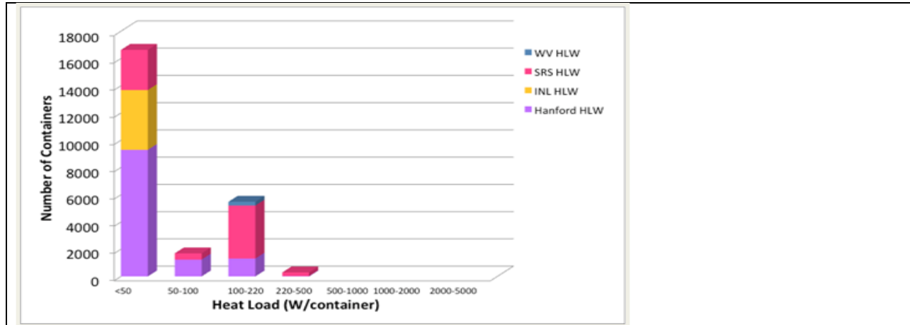
Figure 30: Histogram of DOE High Level Waste (HLW) packages by heat load
