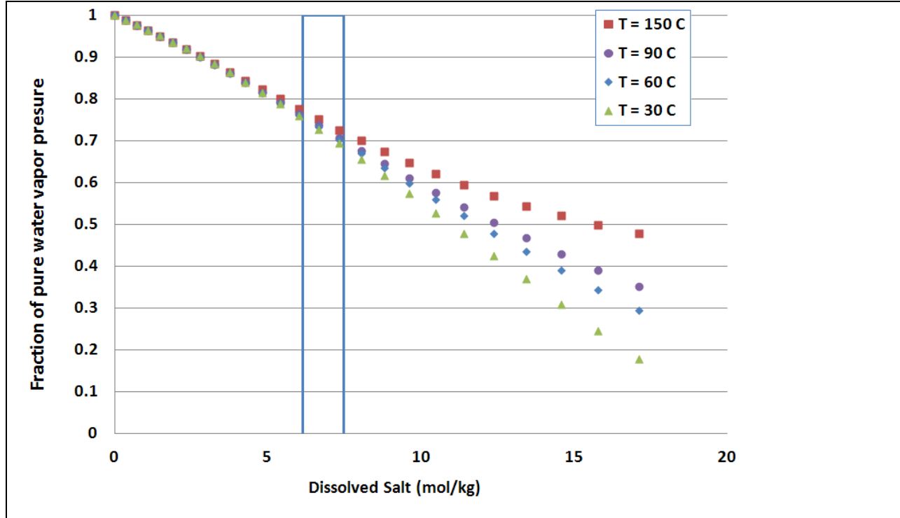
Figure 4: Water vapor pressure (expressed as the fraction of the pure water value) as a function of dissolved salt and temperature, based on functions in Sparrow (2003).
