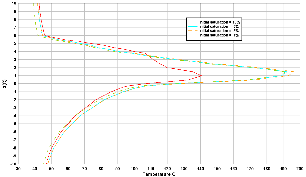
Figure 55: Temperature profile at X=0, Y=0 (zoomed in on the region +/-10 ft of the drift floor) after 2 years for cases with initial saturation varying from A = 1%, B = 3%, C = 5%, and D = 10%. Heat load in all cases is 750W. Z units switched to feet for conformity with the engineering drawings.
