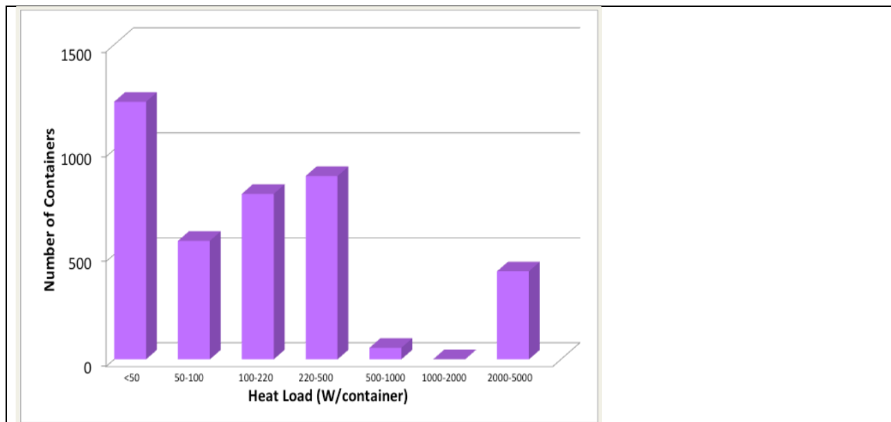
Figure 31: Histogram of DOE Spent Nuclear Fuel (SNF) packages by heat load
