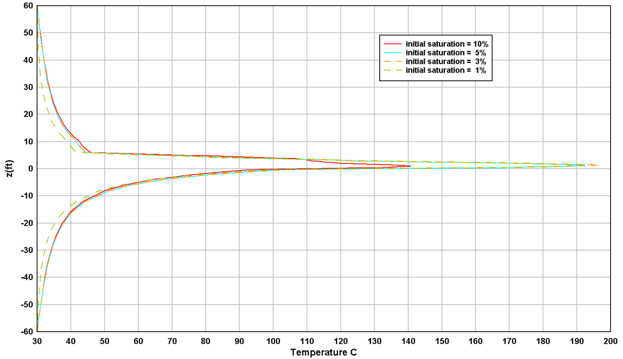
Figure 54: Temperature profile at X=0, Y=0 after 2 years for cases with initial saturation varying from A = 1%, B = 3%, C = 5%, and D = 10%. Heat load in all cases is 750W. Z units switched to feet for conformity with the engineering drawings.
