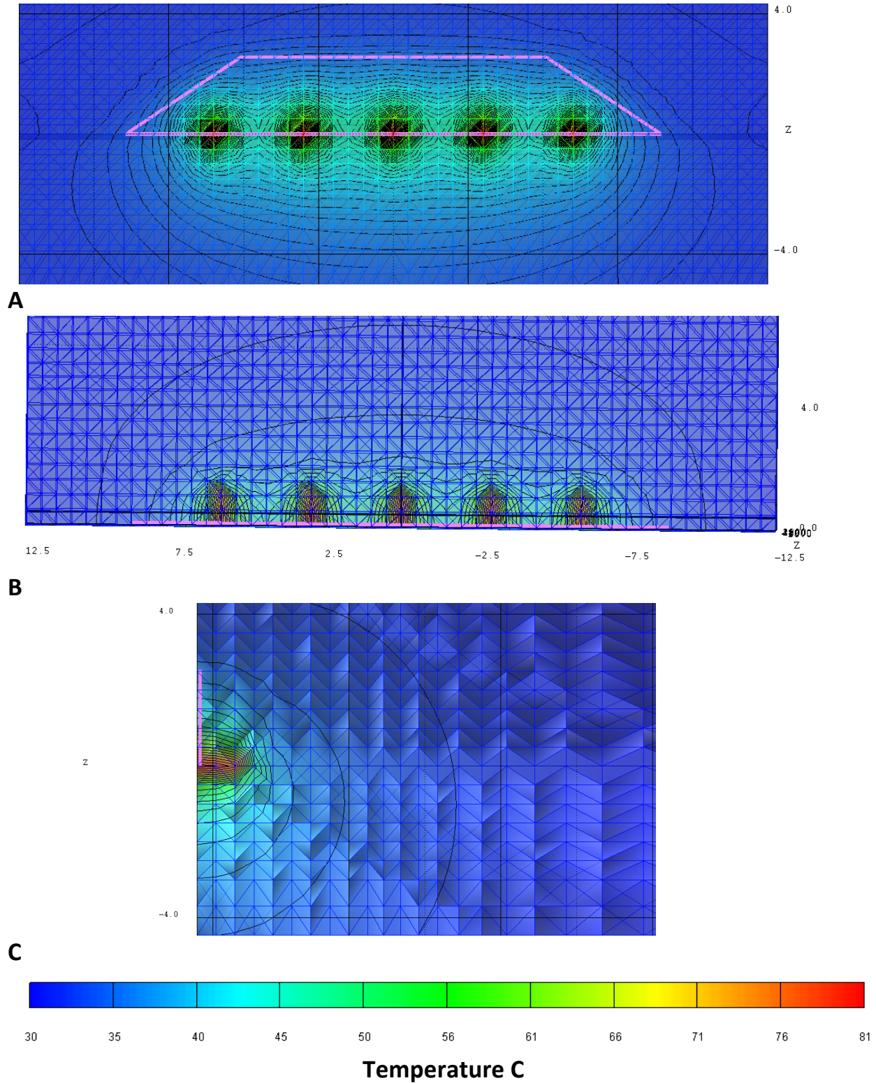
Figure 41: Temperature contours for the 500W case with k=6 \times 10^{-20} \text{ m}^2 on (A) a slice plane x=0.5 \text{ m} ; (B) Z = 0.0 , the floor of the drift slicing through the five heaters, and (C) y = 0 , slicing through the center heater.
