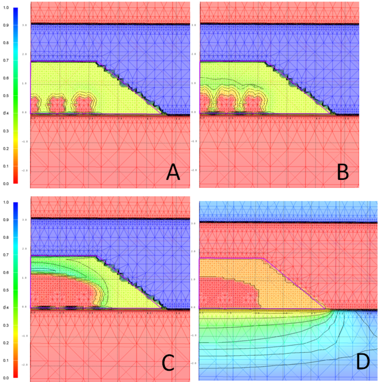
Figure 50: Porosity after 2 years of heating for A) 250W B) 500W and C) 750W per heater. D) Saturation corresponding to the porosity in C.
