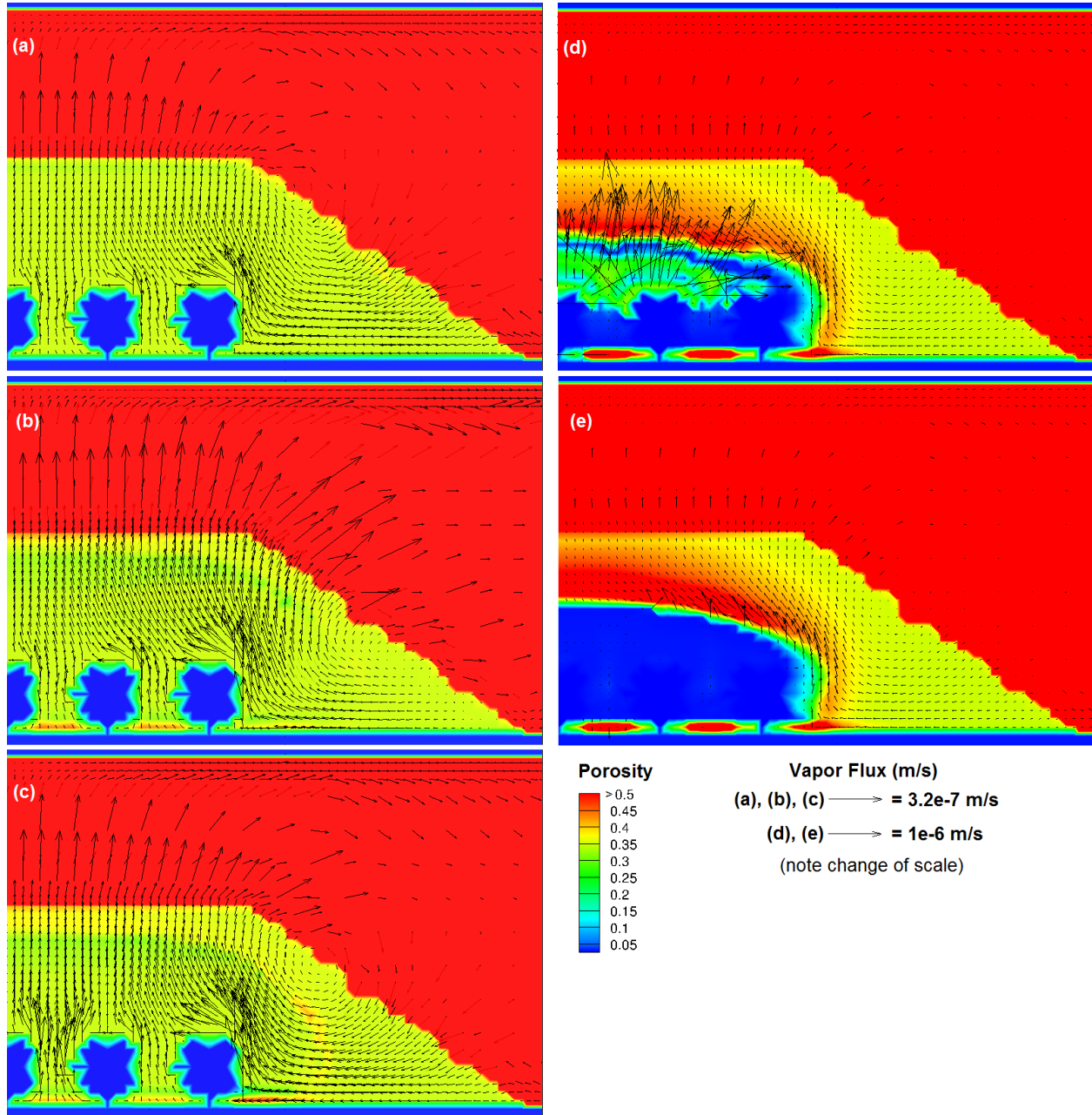
Figure 60: Porosity and vapor flux at 460 days for the following cases: (a) initial saturation of 1%, no clay, maximum suction 0.2 MPa; (b) initial saturation of 1%, 10% clay in crushed salt, maximum suction 0.2 MPa; (c) initial saturation of 5%, no clay, maximum suction 0.2 MPa; (d) initial saturation of 10%, no clay, maximum suction 0.2 MPa; and (e) initial saturation of 10%, no clay, maximum suction 1 MPa.
