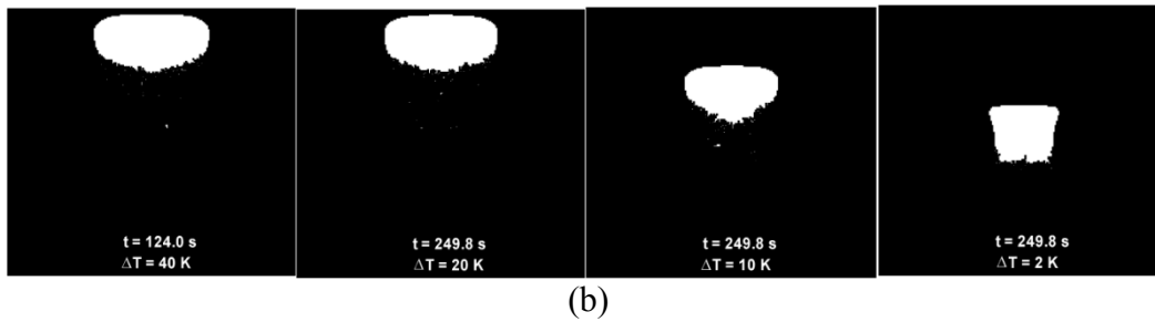
Figure 73: Effects of temperature gradient on the migration process, (a) the relationship between inclusion volume and time, (b) the inclusion shape and location at a given time (249.8 s, except for the leftmost figure, for which the inclusion reaches the boundary at 124 s).
