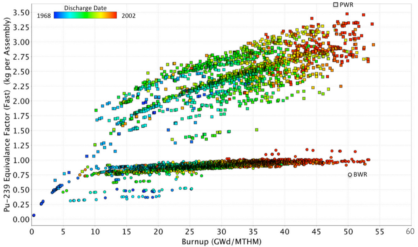
Figure 17. Plutonium-239 equivalence for a fast reactor as a function of burnup, discharged date, and reactor type. Source: Ref. 22.
