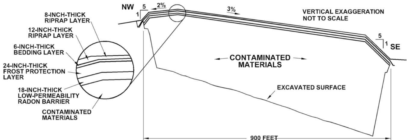
Northwest-Southeast Cross Section of the Slick Rock Disposal Cell.
