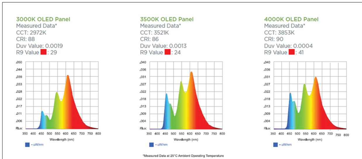
Figure 7. Three color options for OLED panels available from LG Display. Note that the y-axis scale is not identical for all figures. Source: Acuity Brands Lighting, Inc.
