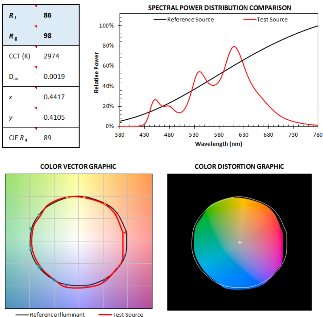
Figure 5. TM-30-15 color metrics and graphics for the LG 3000 K panel used by Acuity Brands Lighting, Inc.
